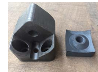
刀座、刀片：CNC加工、模块化设计 Blade holder and blades are CNC processing, Modular design.
